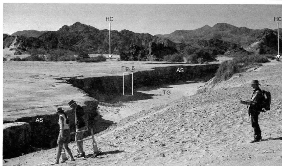
Figure 5. The Amspoort Silts (AS) are characterized by horizontal bedding and deposition in backflooding embayments. The gully is the tributary mouth of the Tsuxub River. The persons are working on the ground penetrating radar (GPR) profile of the site, which was described in detail by Leopold et al. (2006). AS, Amspoort Silts; HC, Hoanib channel, TG, Tsuxub gully
