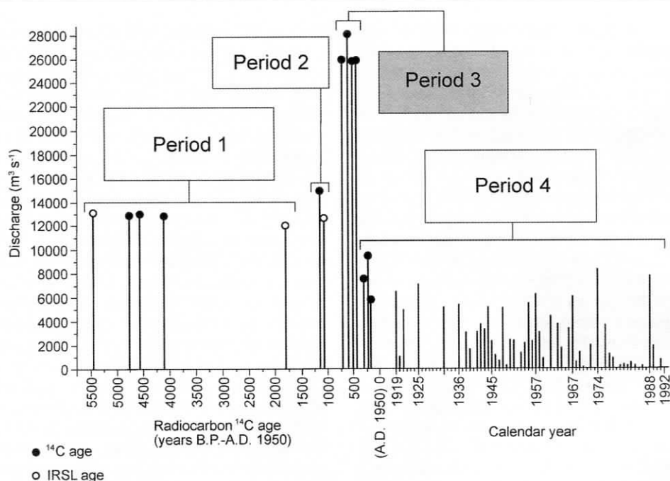
Figure 7. Zawada's (2000) compilation of the palaeoflood record for the lower Orange River [on x-axis left of 0 (A.D. 1950)] and with the annual peak-flow series gauged at Viooldrift for the period 1919–1992 [on x-axis right of 0 (A.D. 1950)]. Zawada (2000) subdivided the entire record into four palaeoflood periods characterized by a threshold discharge value. Period 1: the Orange did not experience a flood that exceeded the threshold discharge of 12,800 \text{ m}^3 \text{ s}^{-1} . Period 2: the Orange did not experience a flood that exceeded the threshold discharge of 14,700 \text{ m}^3 \text{ s}^{-1} . Period 3 (Little Ice Age: four ^{14}\text{C} ages range between AD 1453–AD 1785): the Orange did not experience a flood that exceeded the threshold discharge of 27,000 \text{ m}^3 \text{ s}^{-1} . Period 4: AD 1785–AD 1992; the Orange did not experience a flood that exceeded the threshold discharge of 9,500 \text{ m}^3 \text{ s}^{-1} . By far the most exceptional floods within the past 5,500 ^{14}\text{C} years occurred during the LIA (Period 3)
